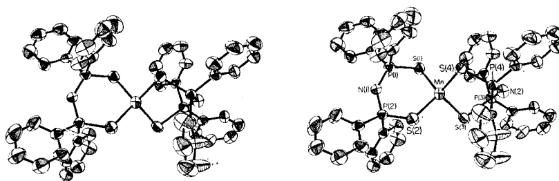
FIGURE 1 Stereoscopic view of the molecular structure of bis(tetraphenyldithioimidodiphosphinato)manganese(II).
