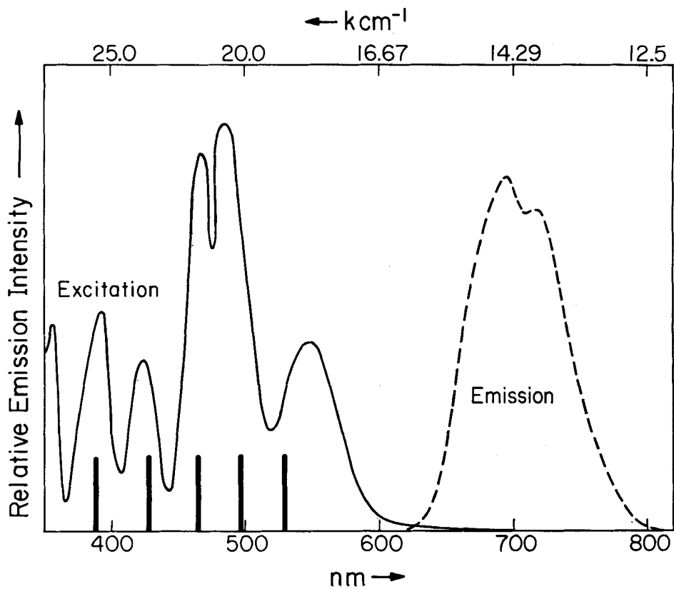
FIGURE 2 Electronic excitation and emission spectra of a solid sample of (1) at 77°K.
